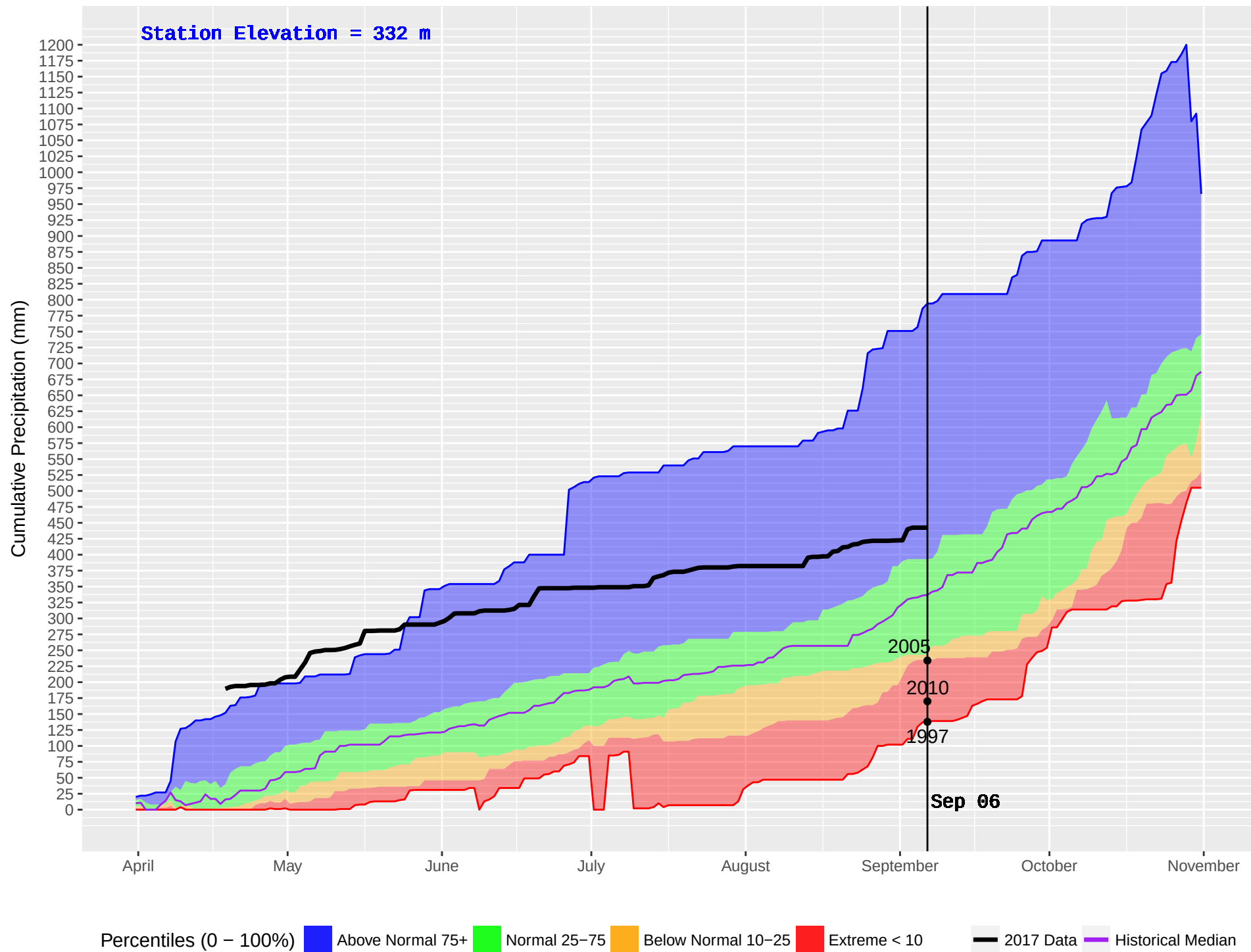
MACHMELL (101) : Historical (1990–2016) and Current (2017) Noon Cumulative Precipitation
