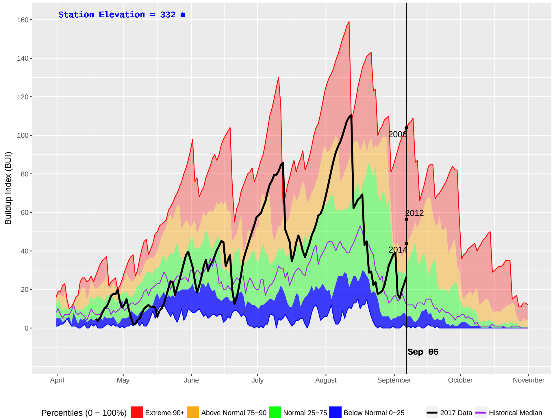
MACHMELL (101) : Historical (1990–2016) and Current (2017) Noon Buildup Index (BUI)
