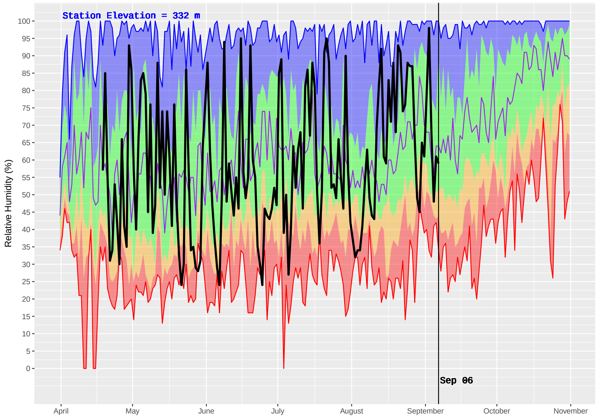
MACHMELL (101) : Historical (1990–2016) and Current (2017) Noon Relative Humidity
