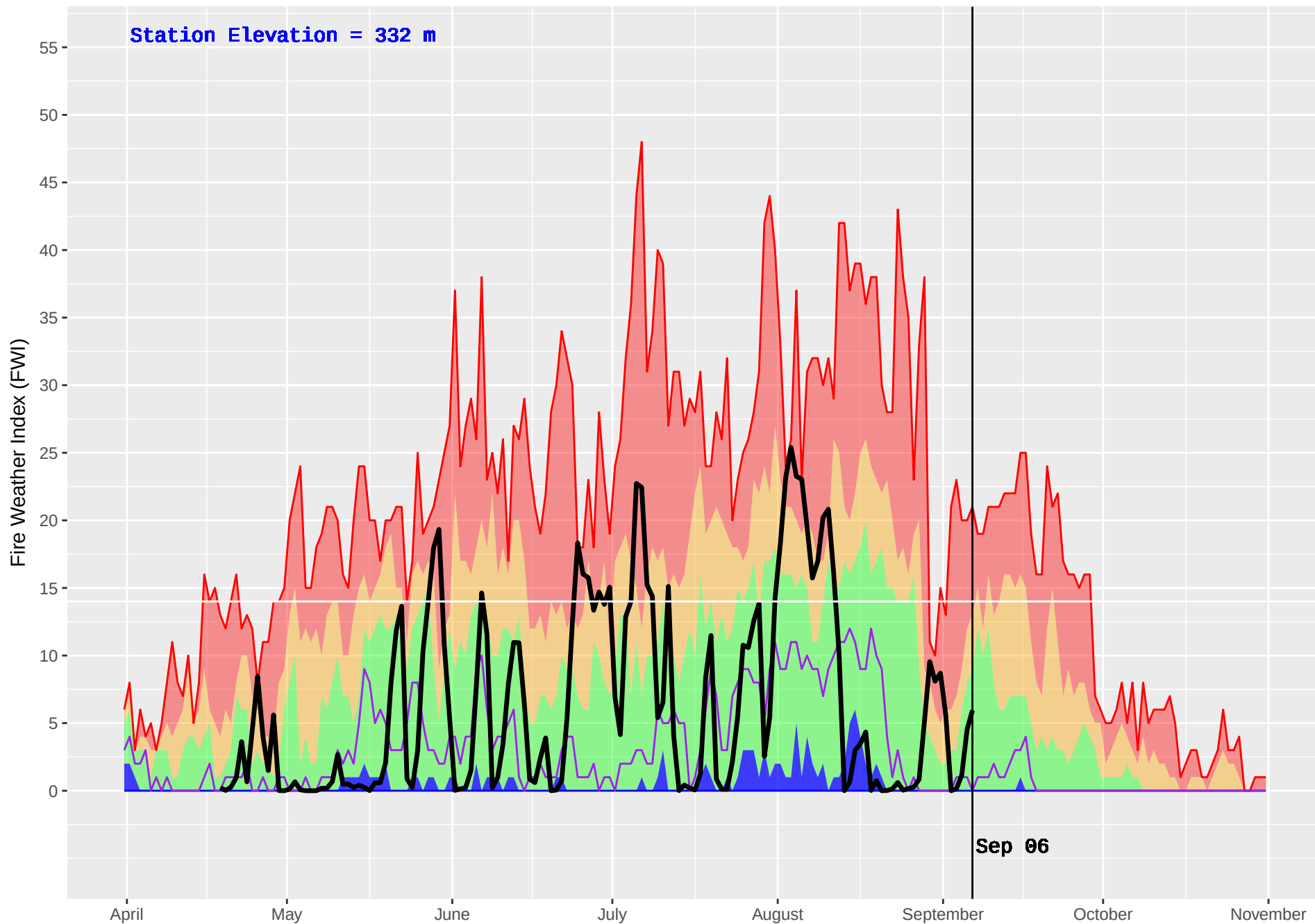
MACHMELL (101) : Historical (1990–2016) and Current (2017) Noon Fire Weather Index (FWI)
