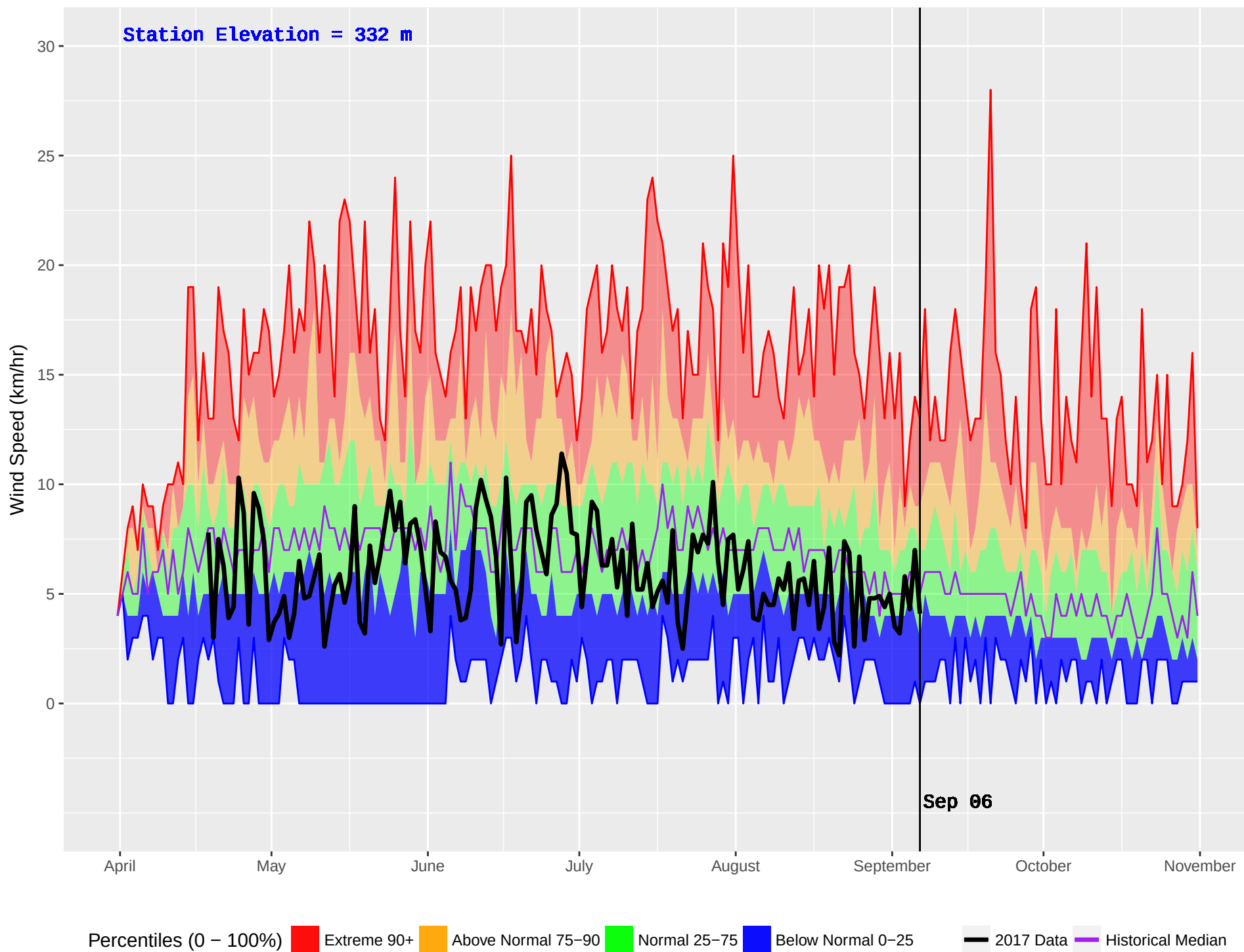
MACHMELL (101) : Historical (1990–2016) and Current (2017) Noon Wind Speed
