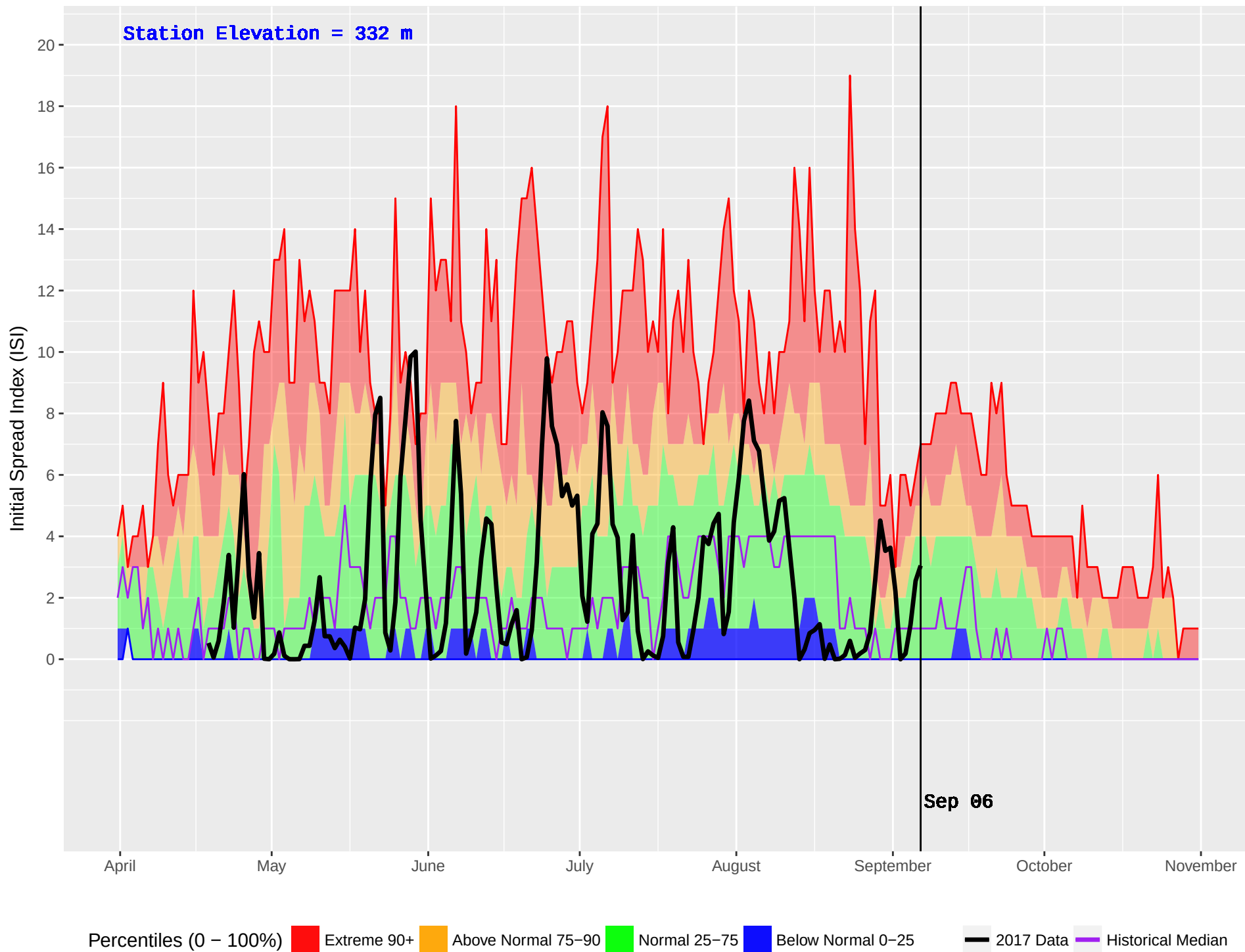
MACHMELL (101) : Historical (1990–2016) and Current (2017) Noon Initial Spread Index (ISI)
