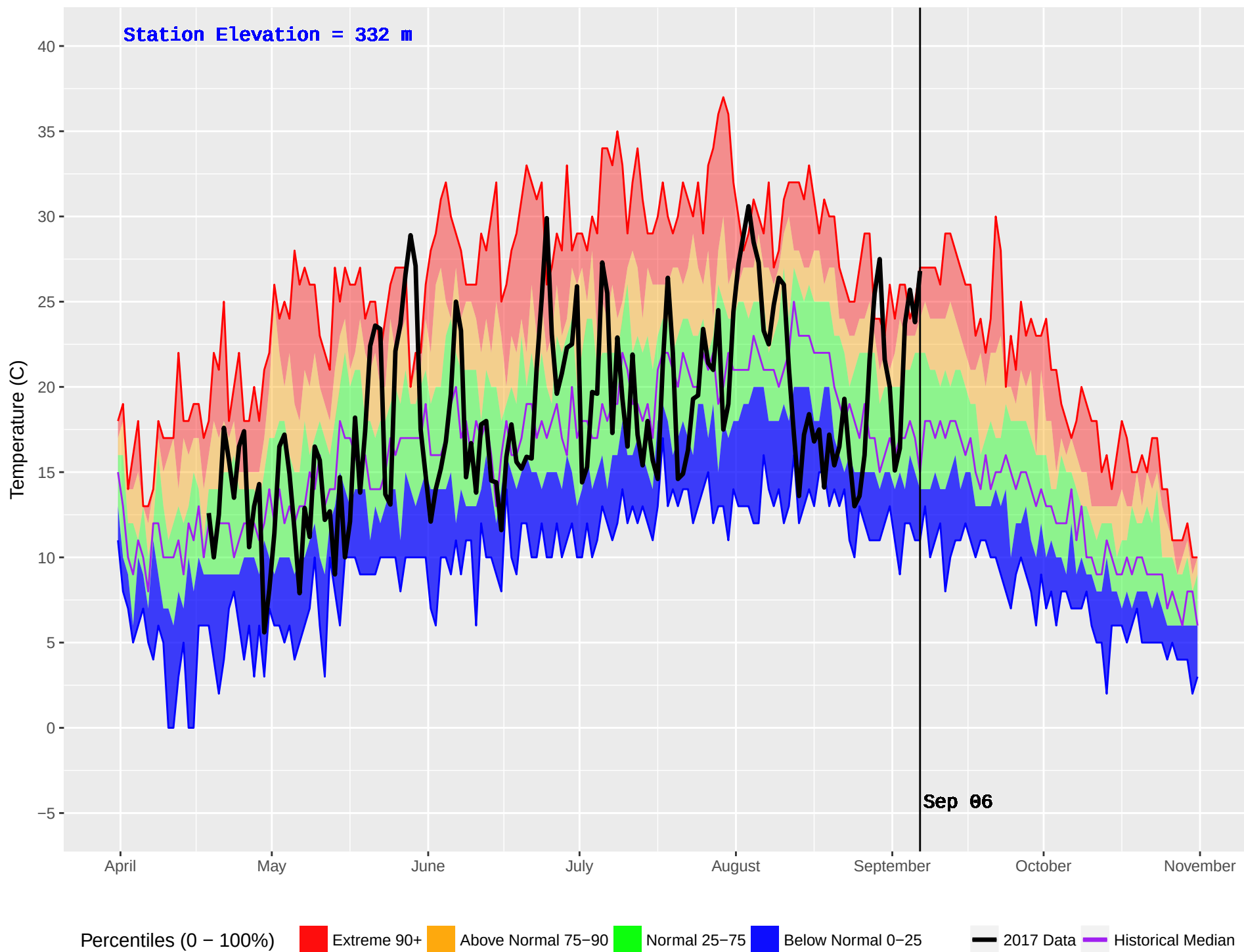
MACHMELL (101) : Historical (1990–2016) and Current (2017) Noon Temperature
